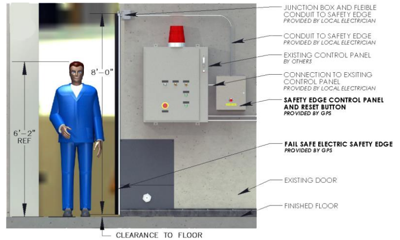
Safety Edge Retro-Fit System Layout, Elevation View Acoustic Elephant Door Example
